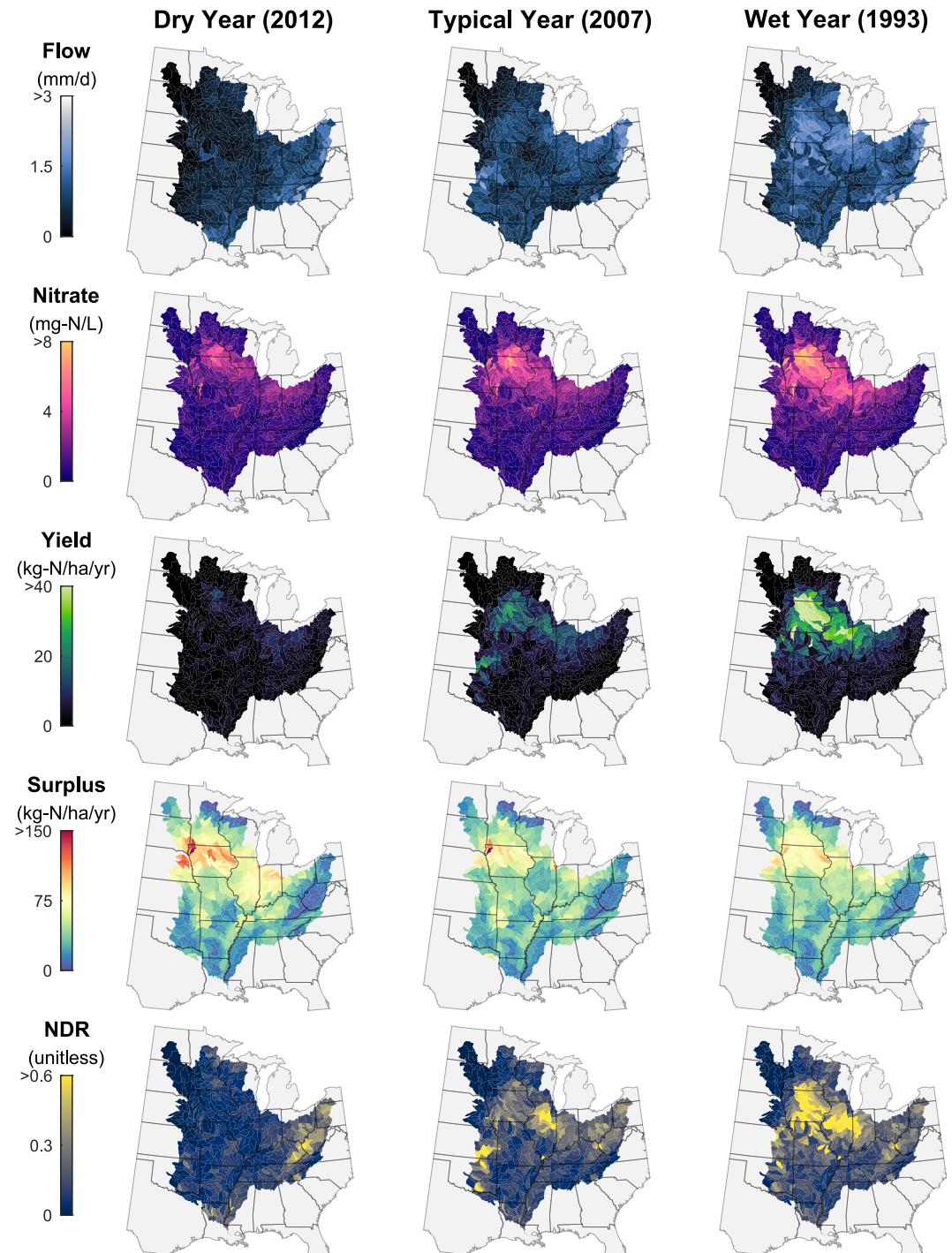
Figure 8. Model results for a dry year (2012), a typical year (2007), and a wet year (1993) in the MRB study domain. The upper Midwestern states, like Illinois, Iowa, and Minnesota, experience the greatest sensitivity of nitrate yield and delivery in response to regional-scale hydrology. NDR, Nitrogen Delivery Ratio.
